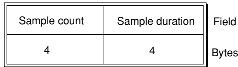
Figure 2-29 The layout of a time-to-sample table entry
